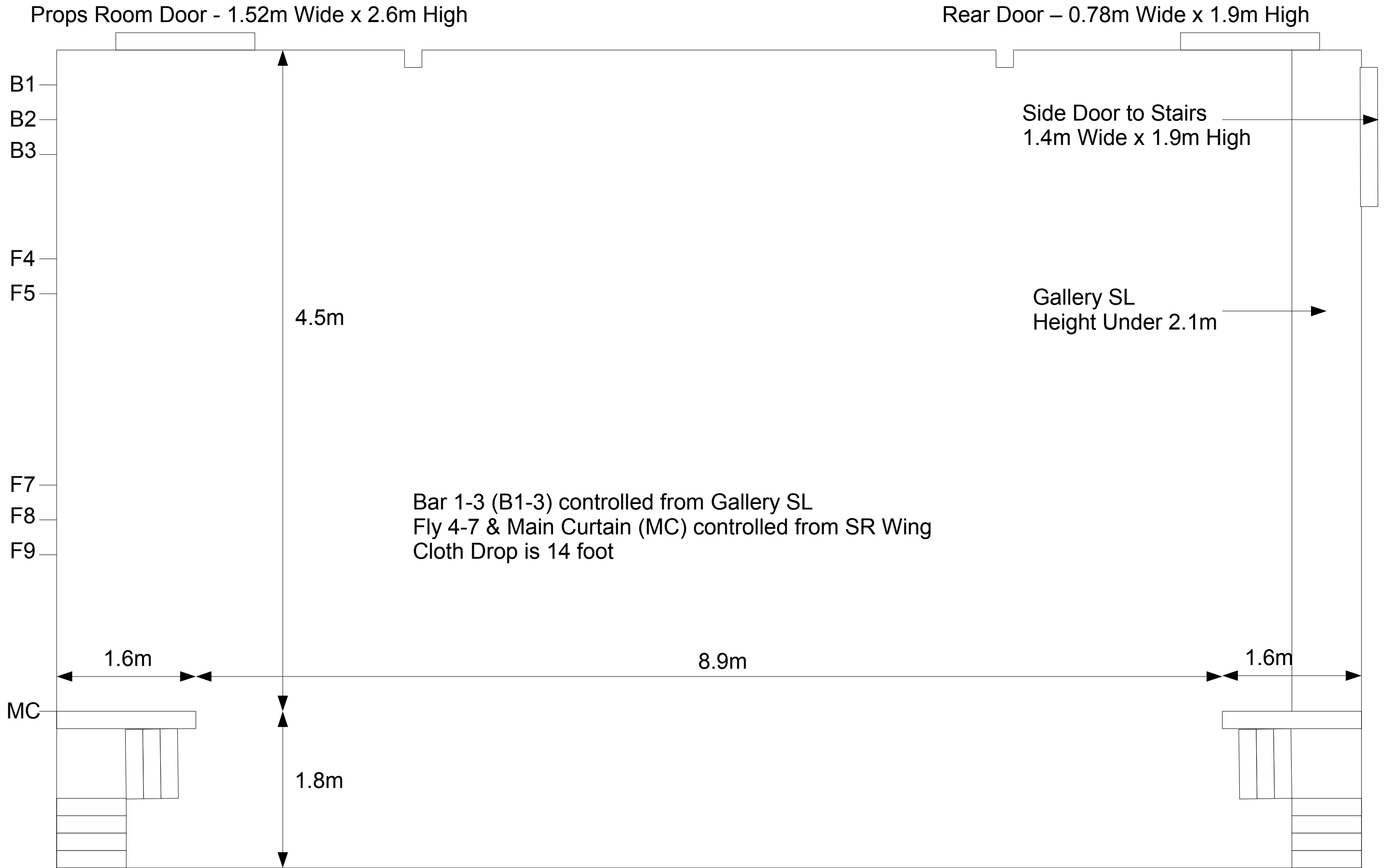
Frodsham Community Centre Main Stage – Dimensions & Notes (Sep 2022)
